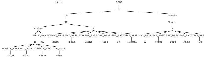
Figure 5. C-structure tree for (7) (sublexical morphology shown)
